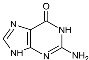
Guanina (G)
